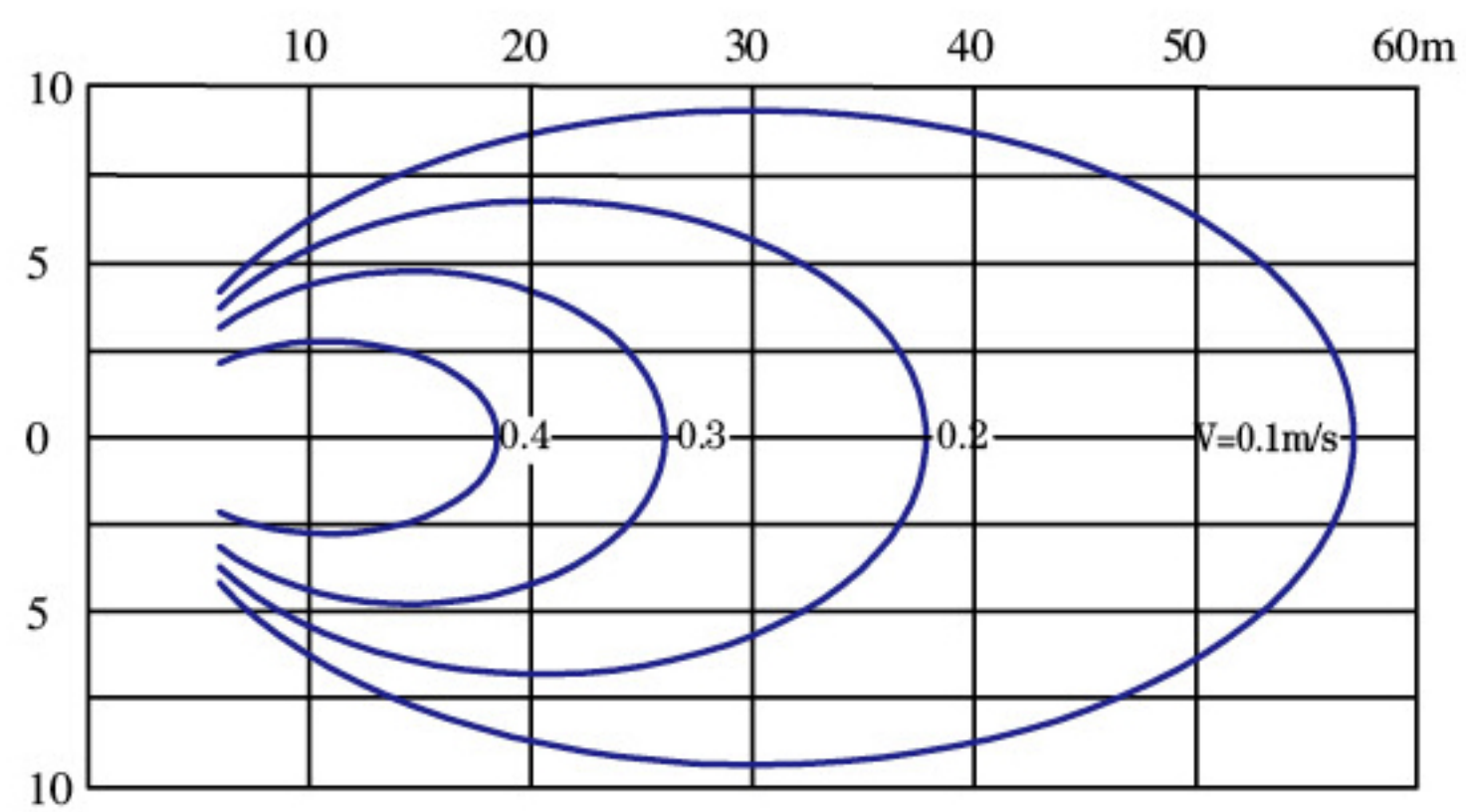
QDTM1080/102/3-3
