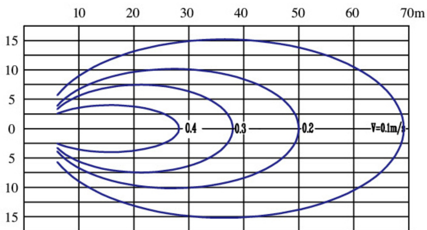
QDTM1080/121/3-5.5
